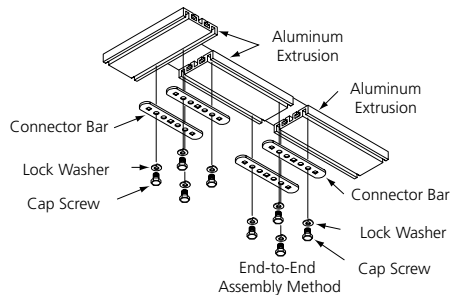
Aluminum Track Support Kit (FGS-HASK-C)
